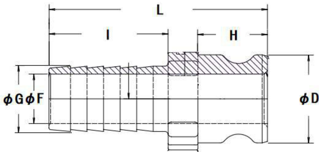
Section B-B
